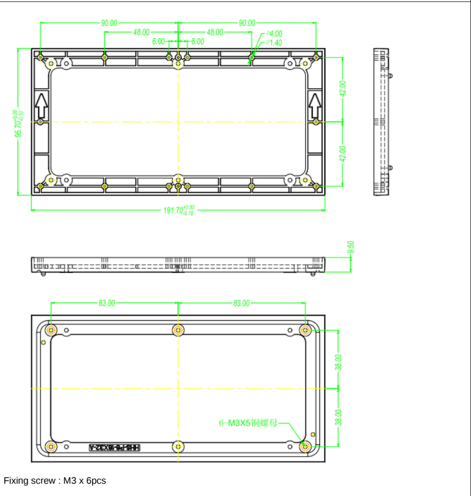
( 5 ) Drawing of the frame
